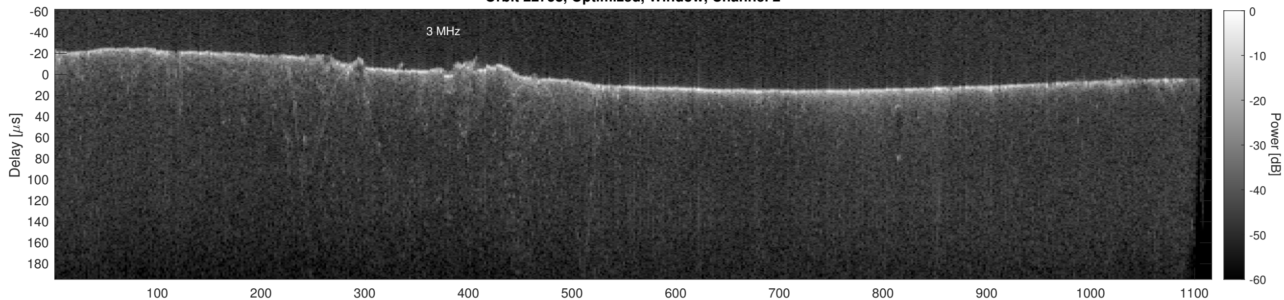
Orbit 22758, Cluttergram
