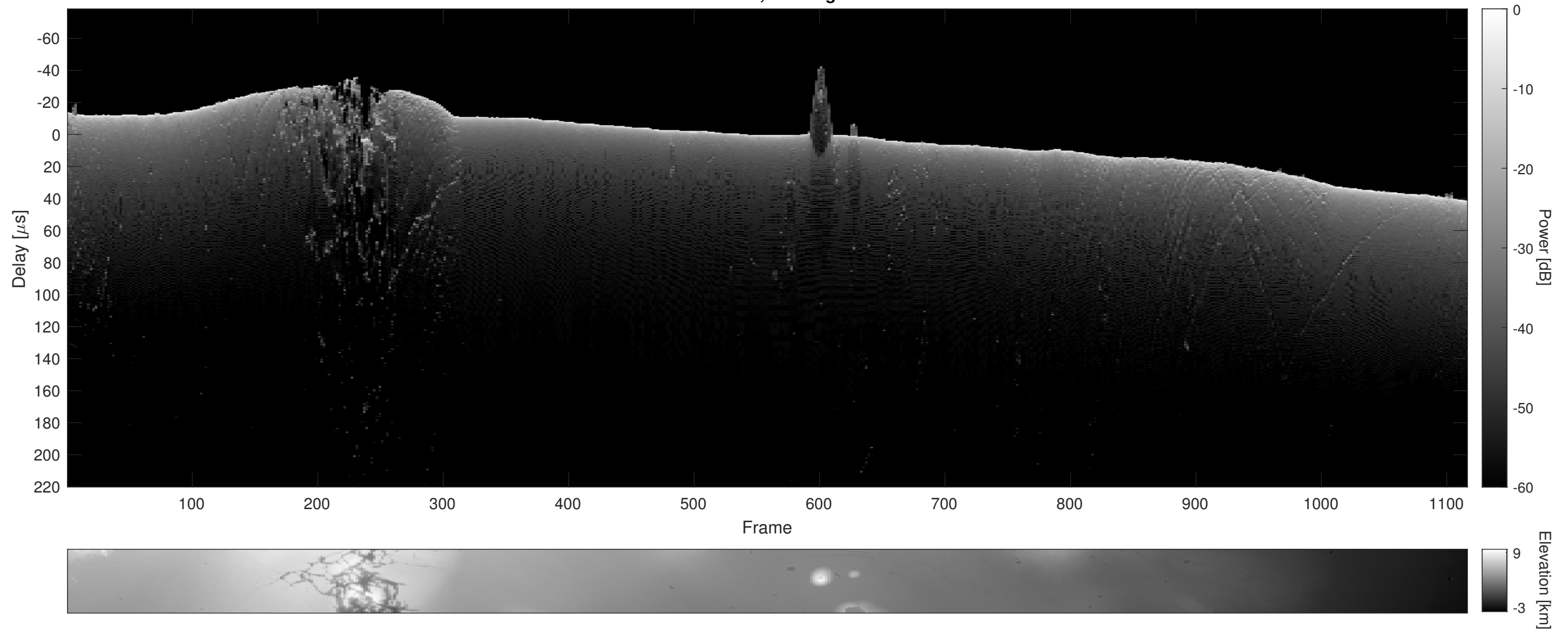
Orbit 22760, Cluttergram
