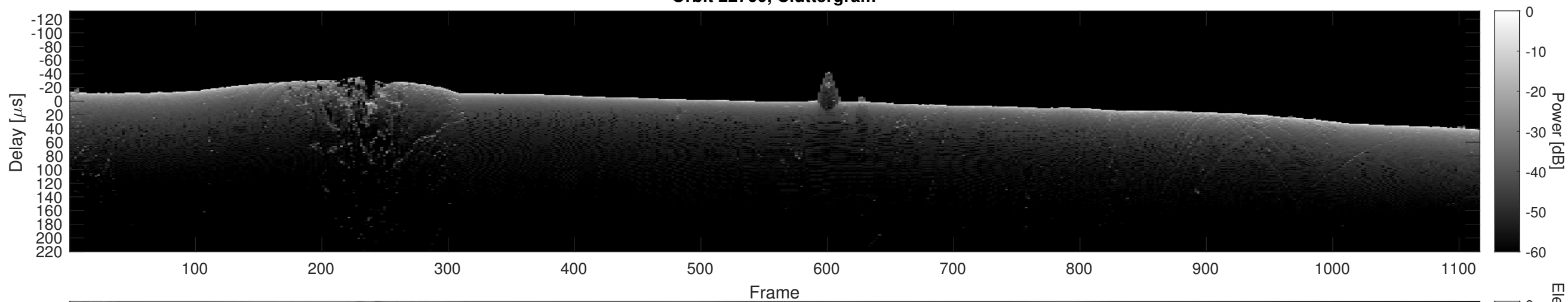
Orbit 22760, Cluttergram
