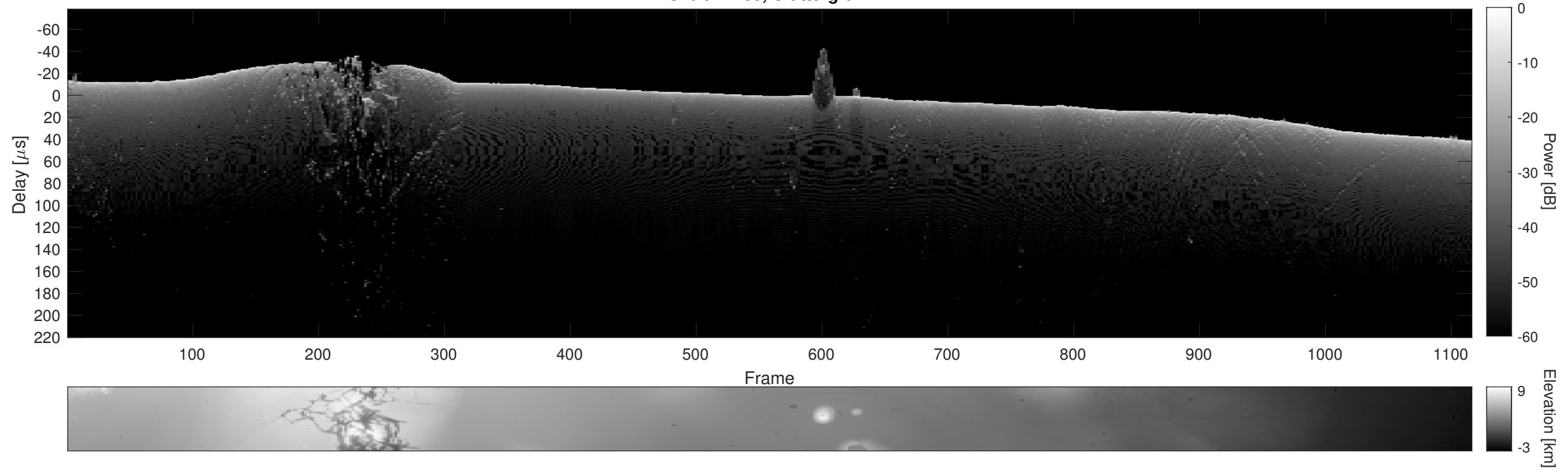
Orbit 22760, Cluttergram
