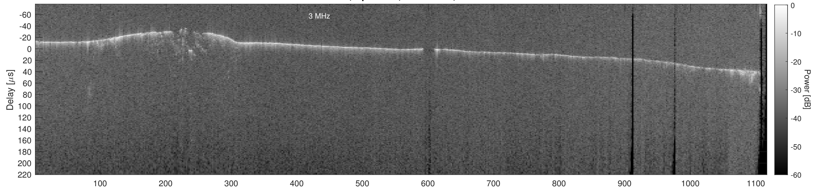
Orbit 22760, Cluttergram
