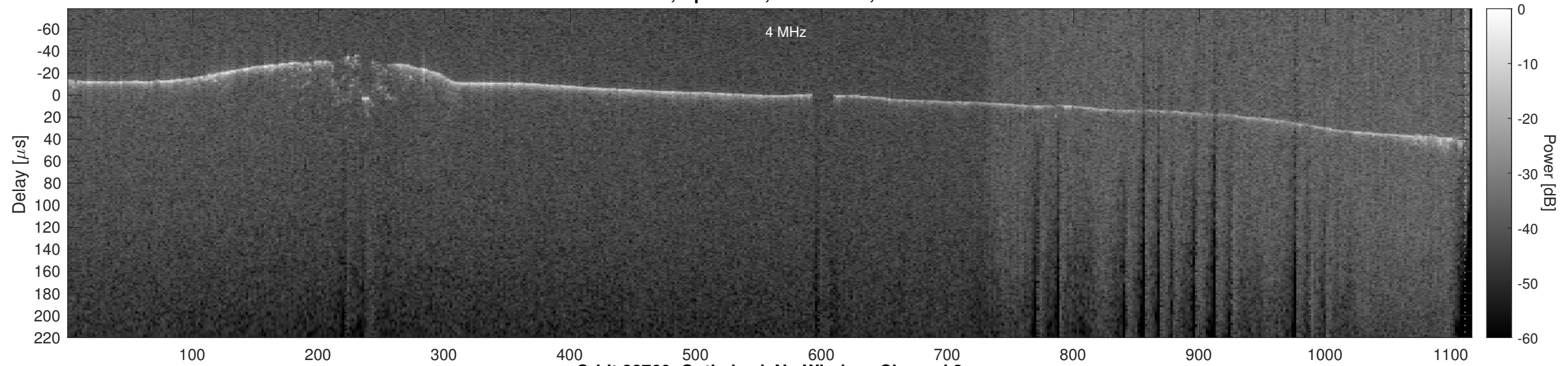
Orbit 22760, Optimized, No Window, Channel 2
