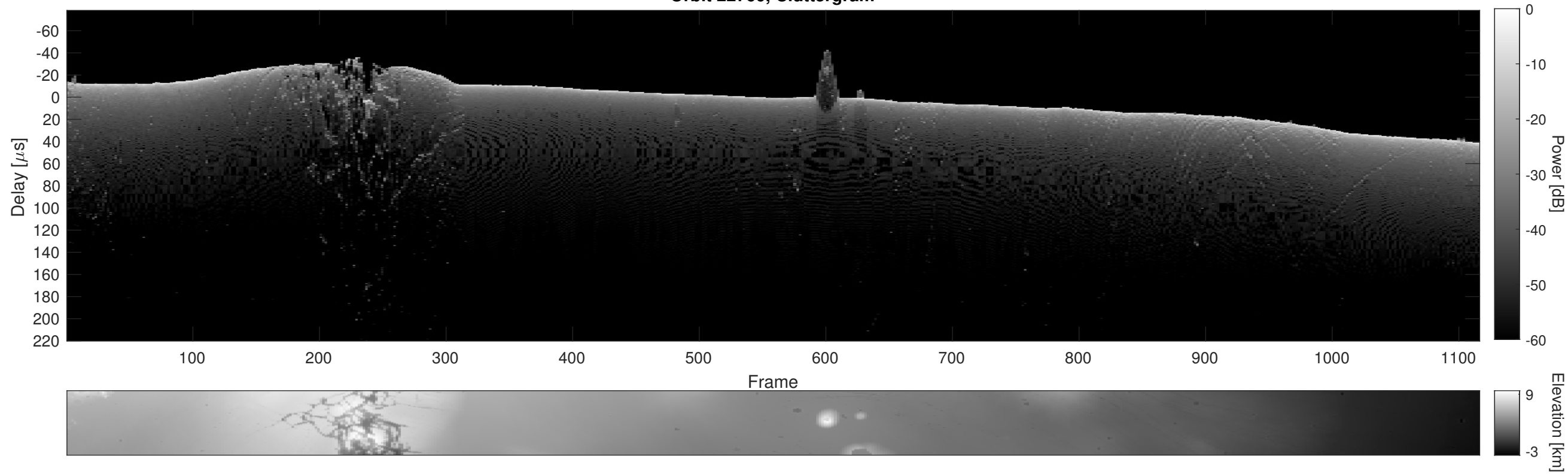
Orbit 22760, Cluttergram
