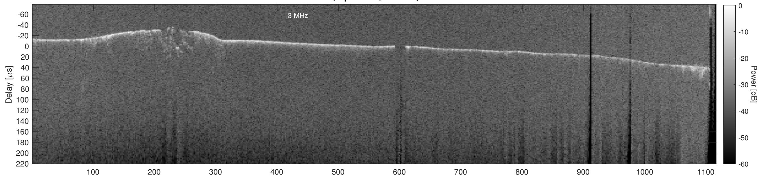
Orbit 22760, Cluttergram
