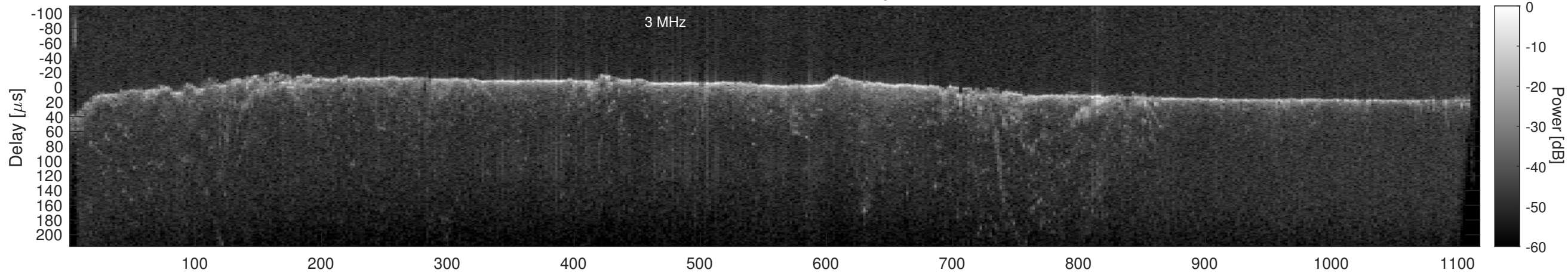
Orbit 22762, Cluttergram
