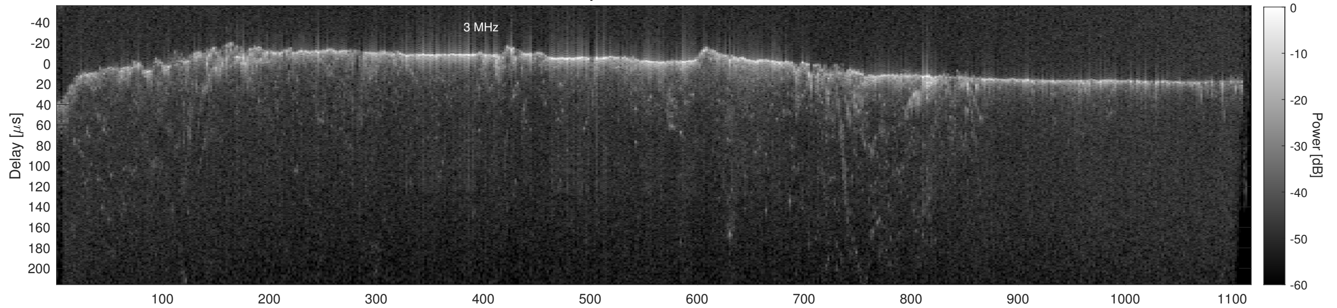
Orbit 22762, Cluttergram
