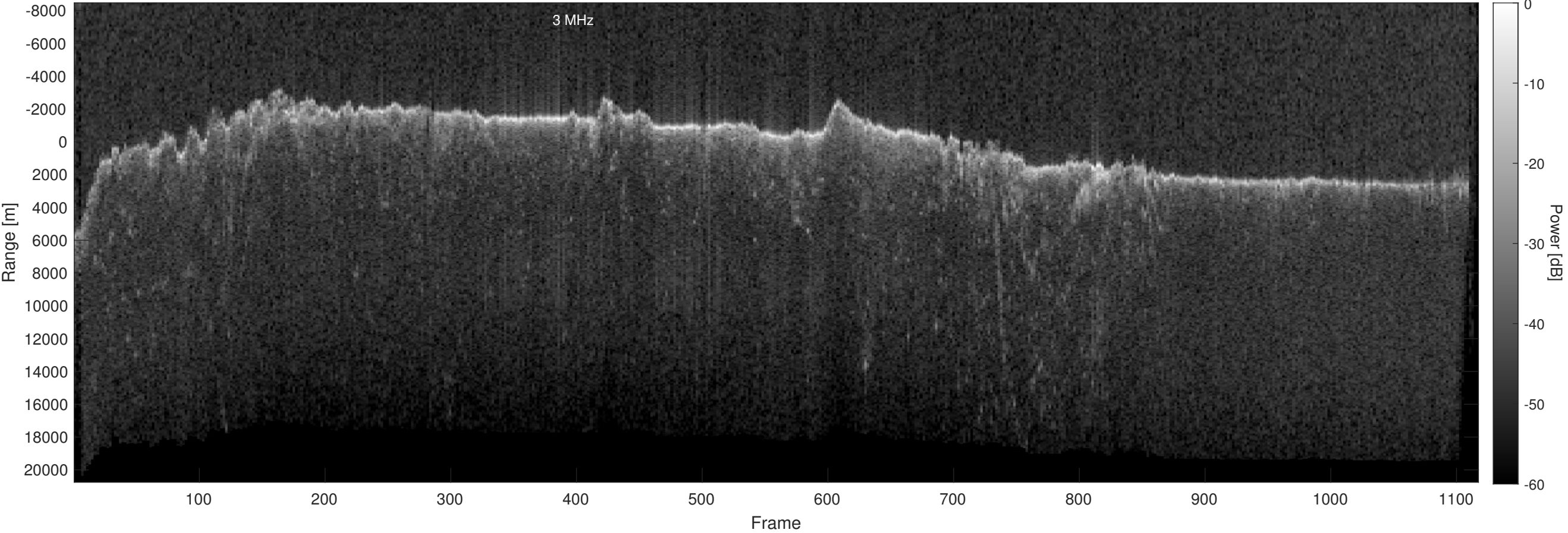
Orbit 22762, Optimized, Window, Depth-Corrected, Channel 2
