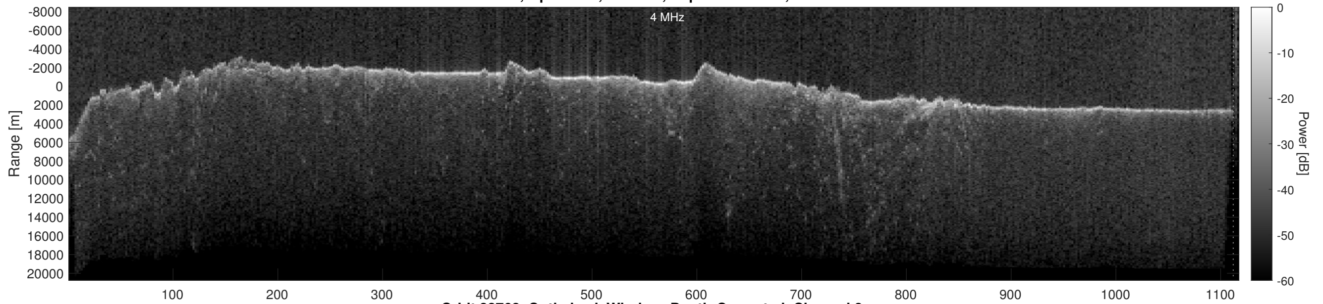
Orbit 22762, Optimized, Window, Depth-Corrected, Channel 2
