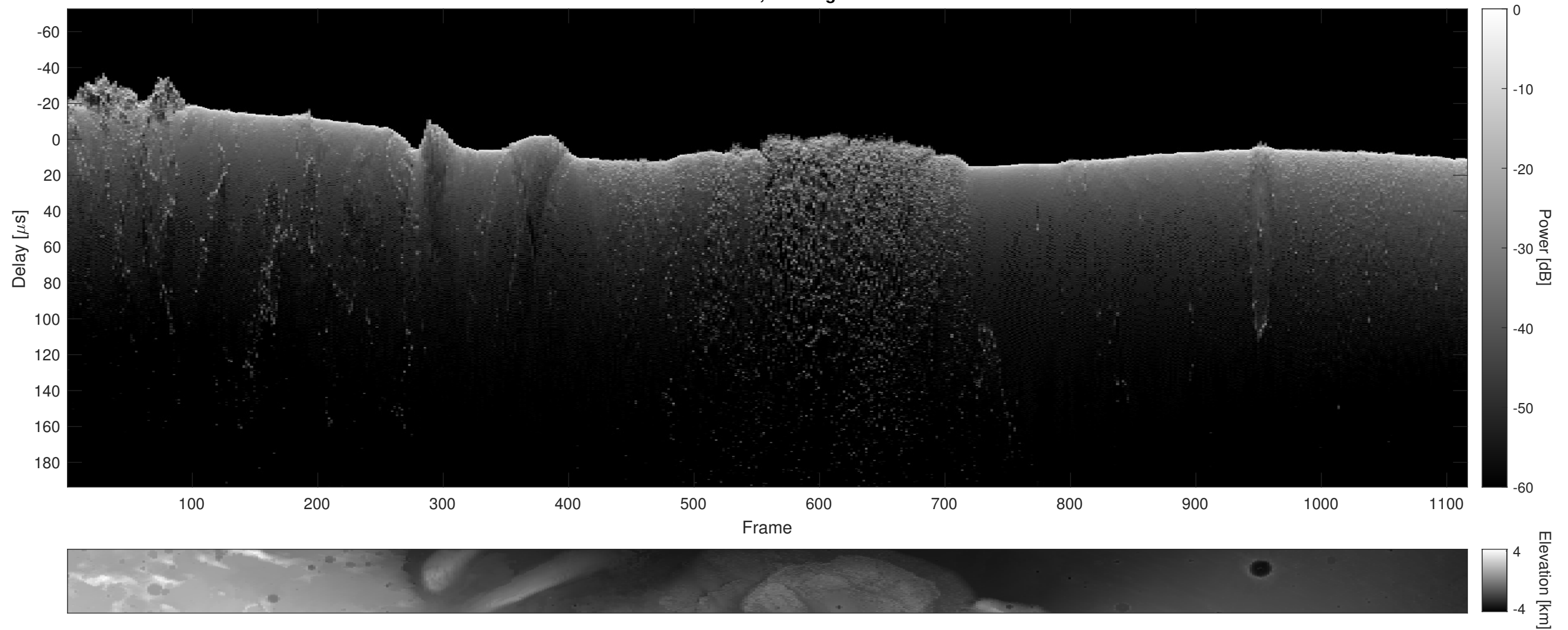
Orbit 22764, Cluttergram
