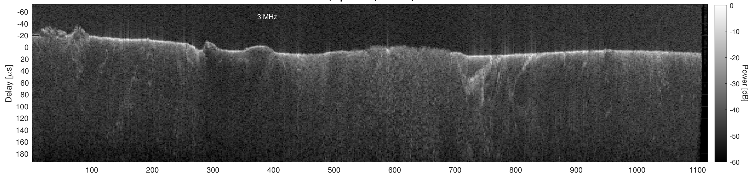
Orbit 22764, Cluttergram
