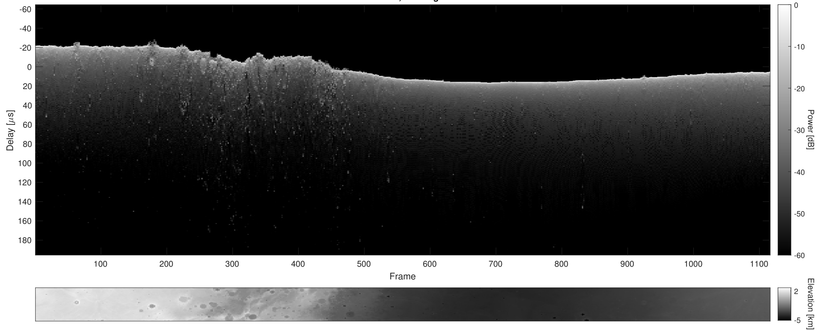
Orbit 22765, Cluttergram
