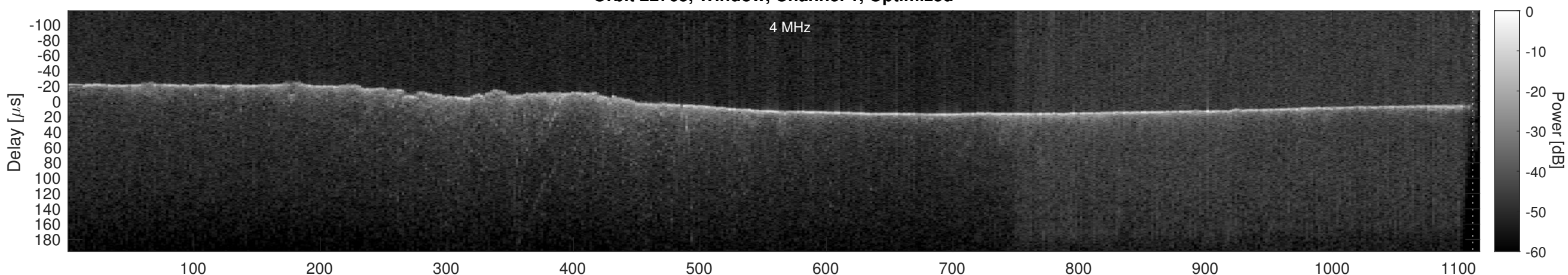
Orbit 22765, Cluttergram
