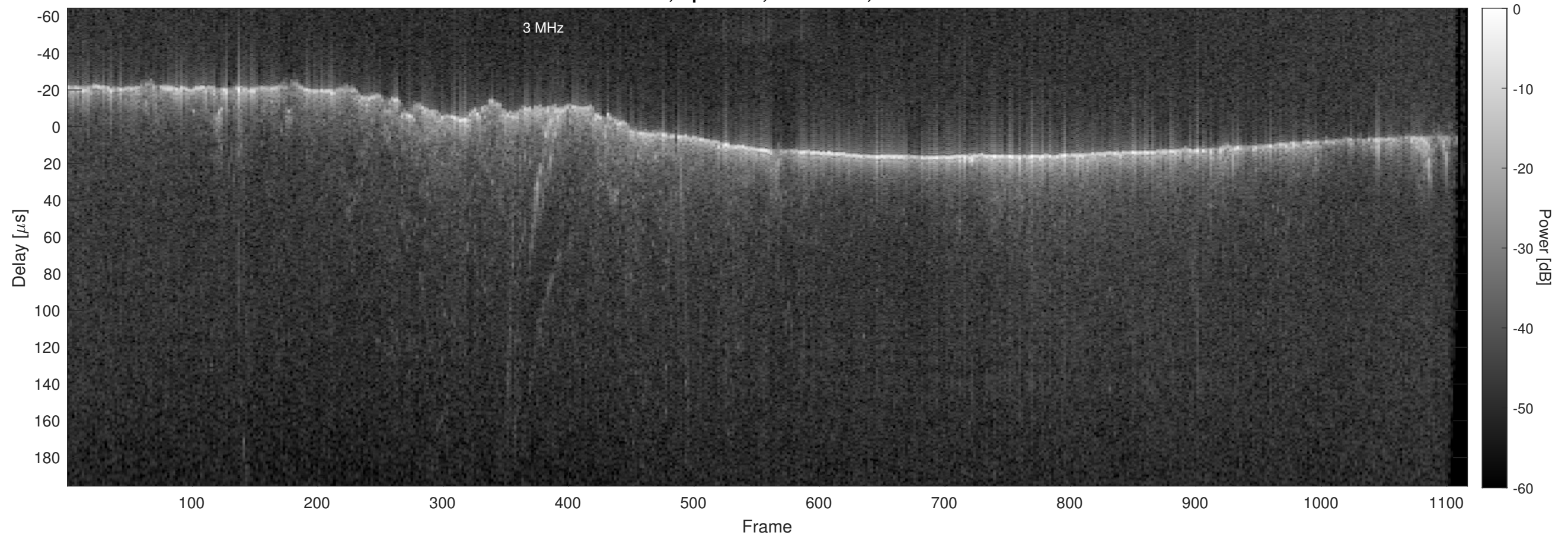
Orbit 22765, Optimized, No Window, Channel 2
