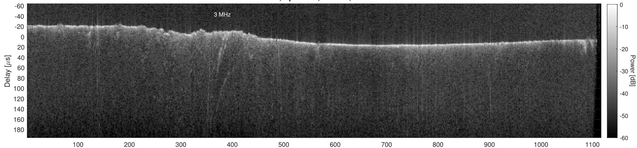
Orbit 22765, Cluttergram
