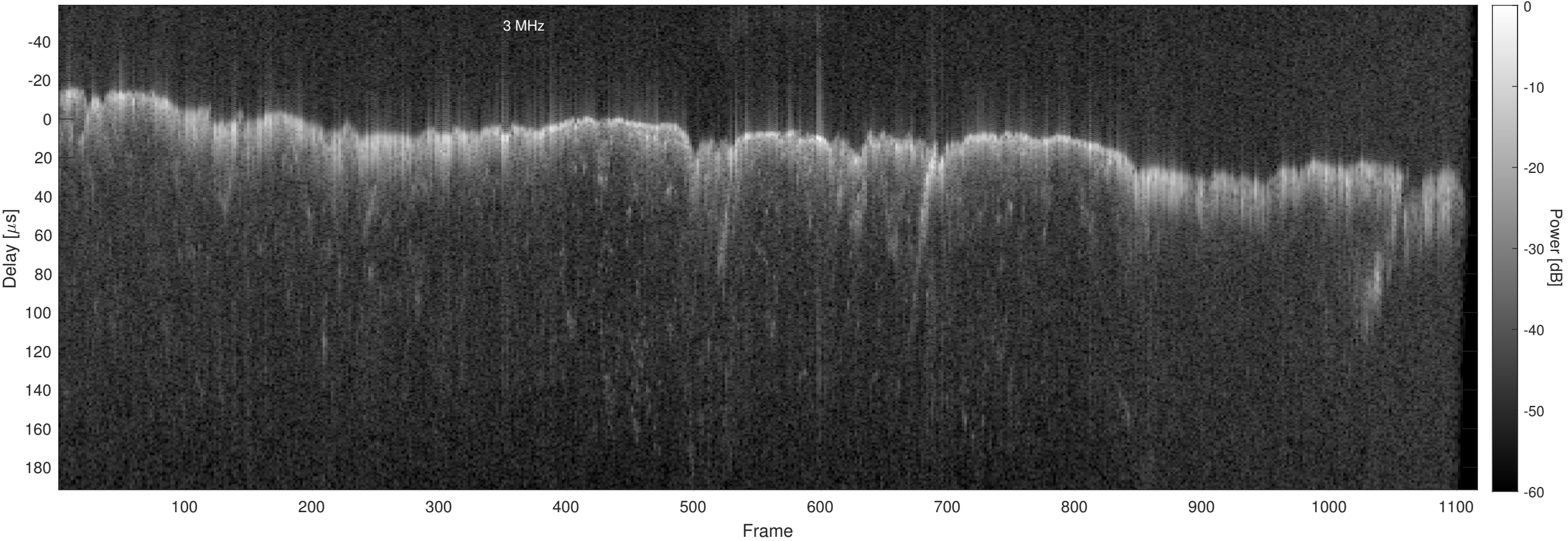
Orbit 22766, Chapman, No Window, Channel 2
