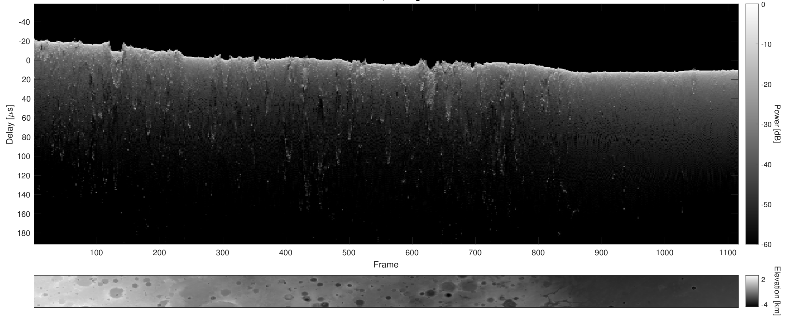
Orbit 22766, Cluttergram
