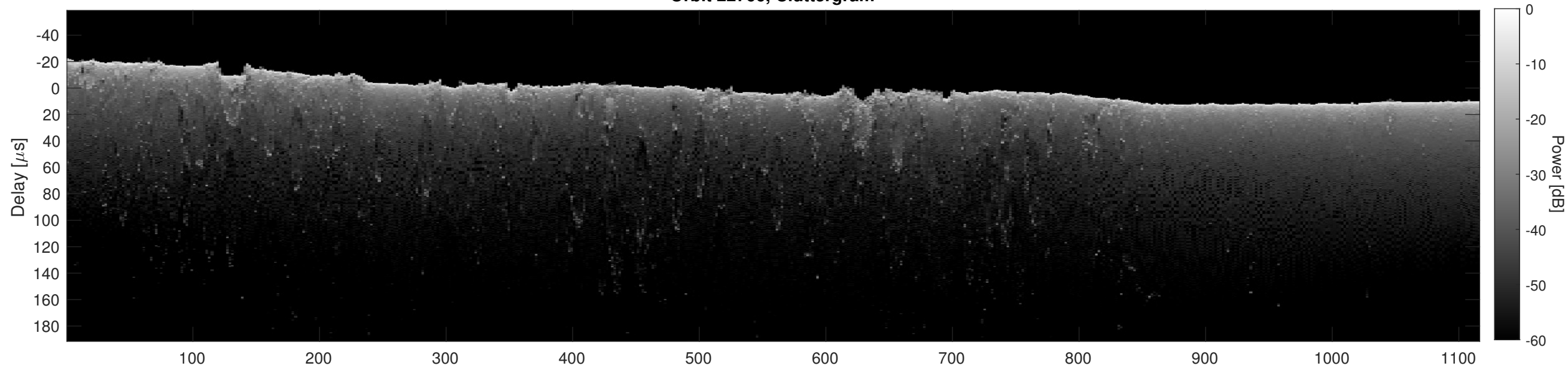
Orbit 22766, Cluttergram
