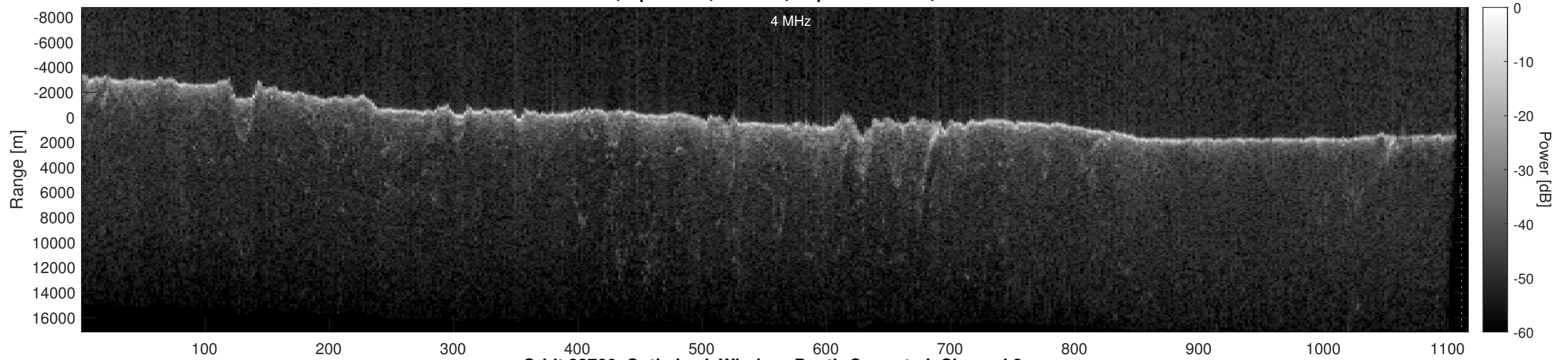
Orbit 22766, Optimized, Window, Depth-Corrected, Channel 2
