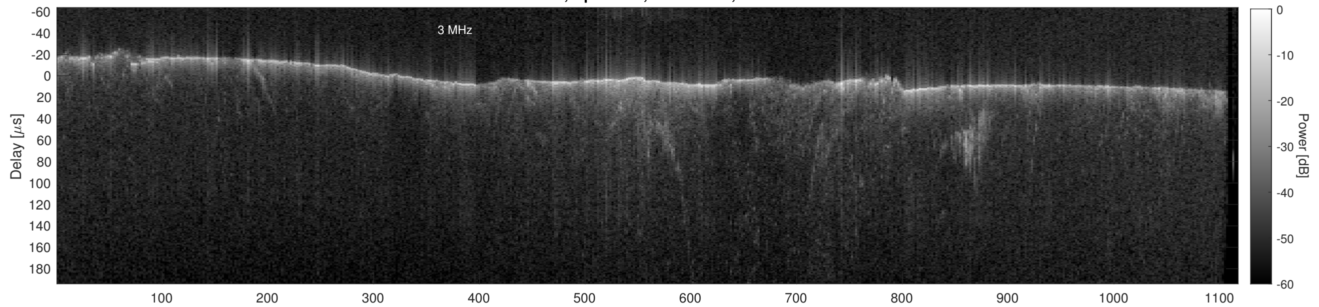
Orbit 22771, Cluttergram
