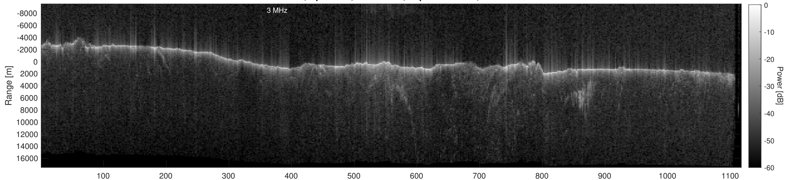
Orbit 22771, Depth-Corrected Cluttergram
