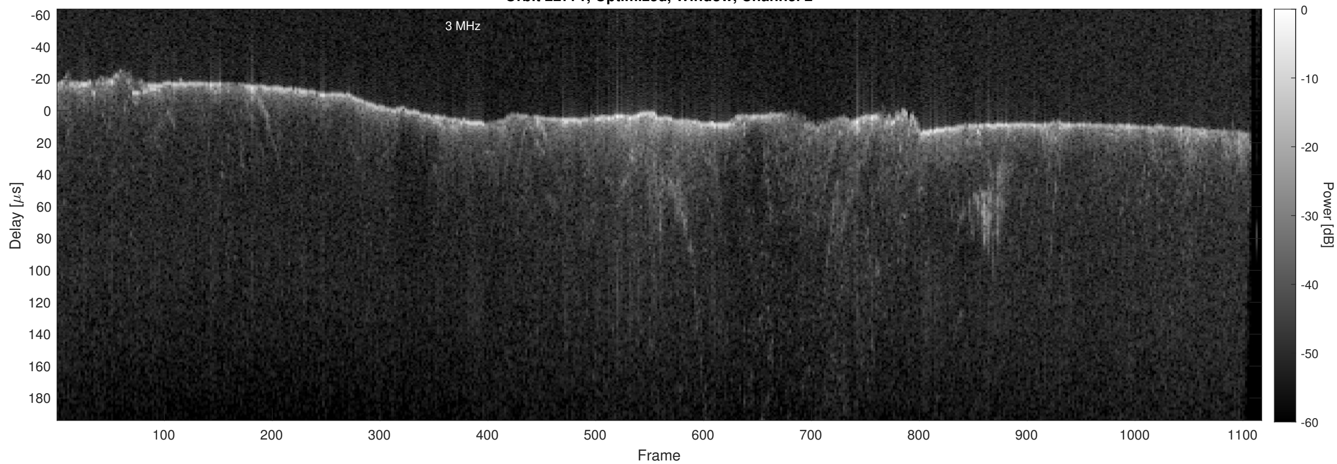
Orbit 22771, Optimized, Window, Channel 2
