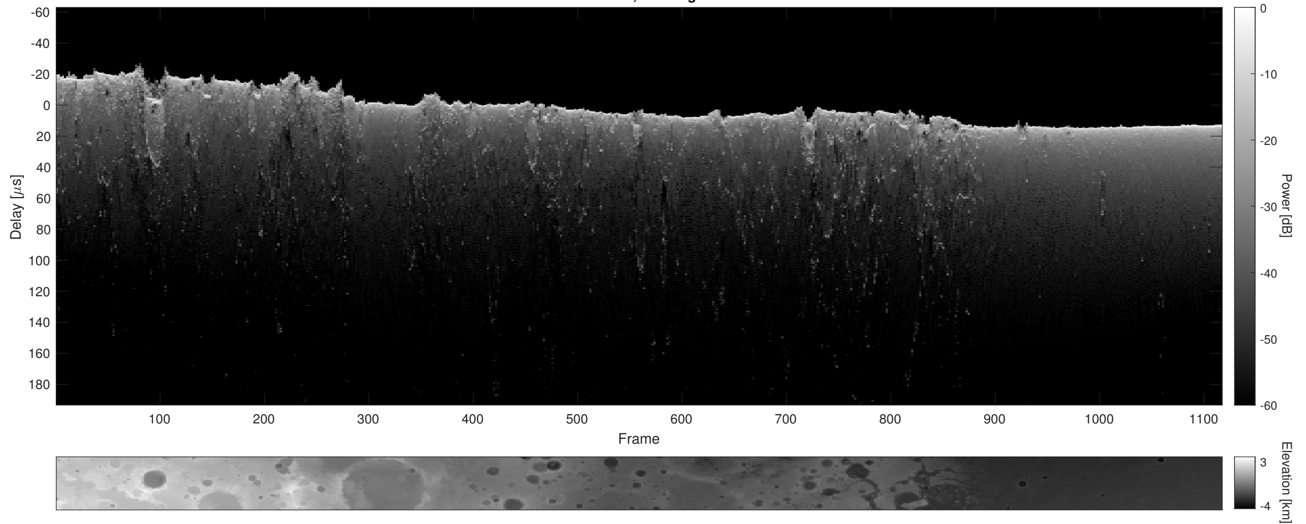
Orbit 22773, Cluttergram
