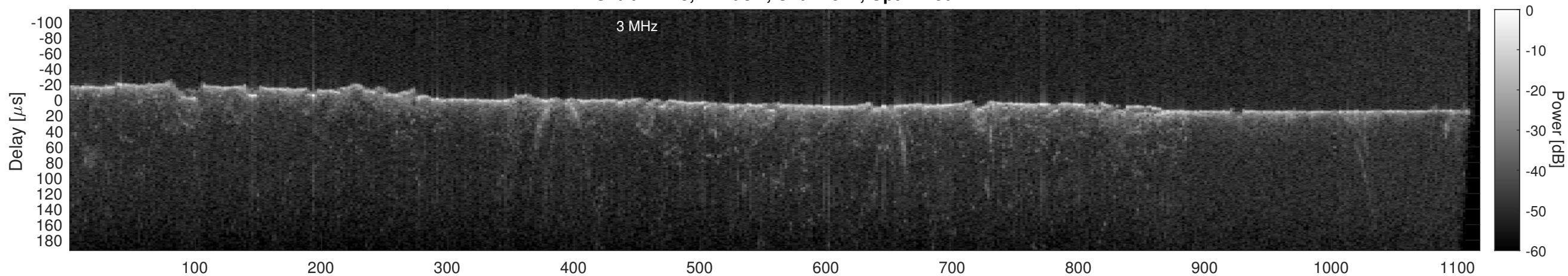
Orbit 22773, Cluttergram
