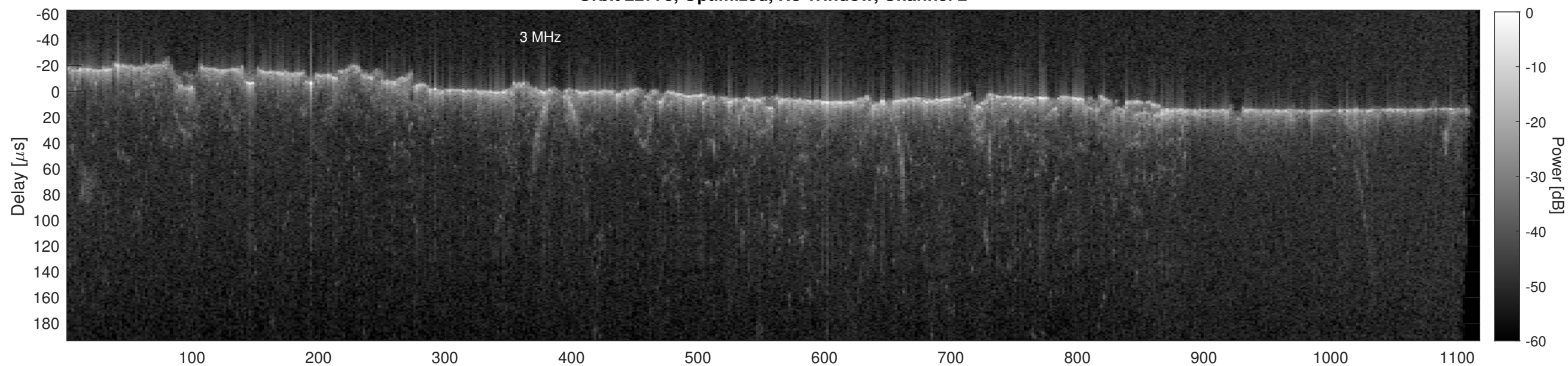
Orbit 22773, Cluttergram
