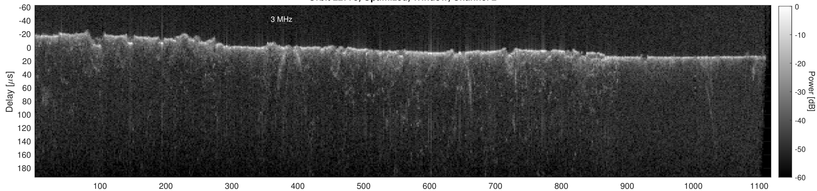
Orbit 22773, Cluttergram
