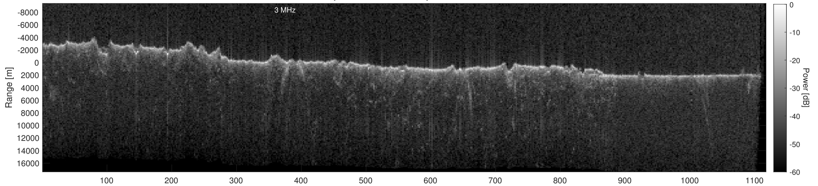
Orbit 22773, Depth-Corrected Cluttergram
