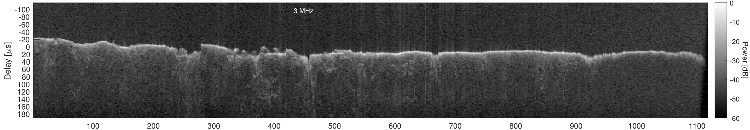
Orbit 22777, Window, Channel 2, Chapman
