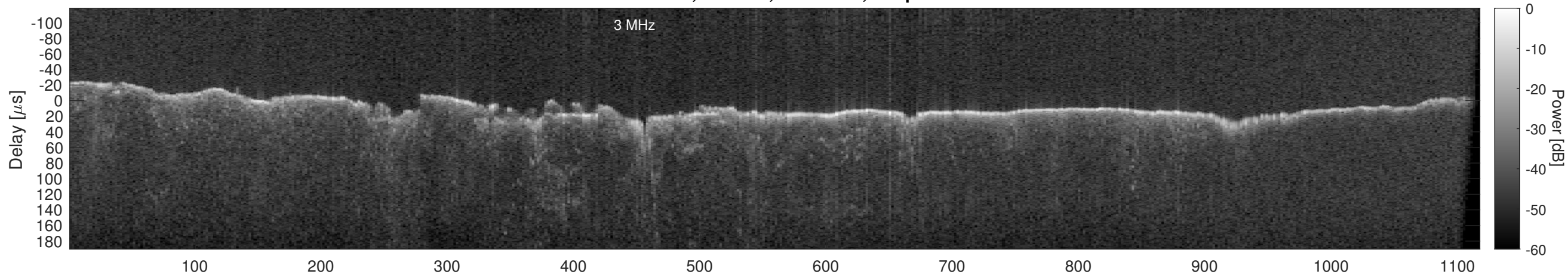
Orbit 22777, Window, Channel 2, Optimized
