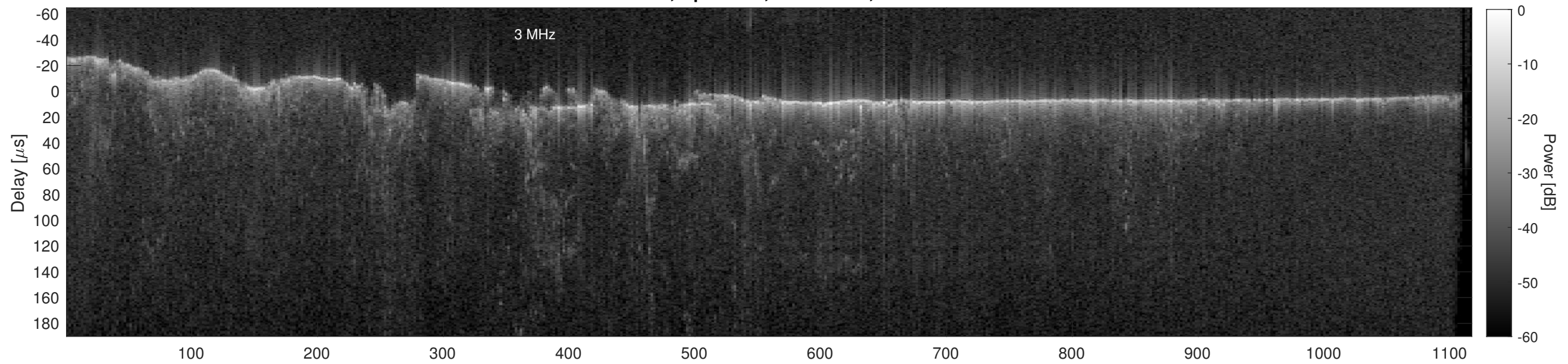
Orbit 22777, Cluttergram
