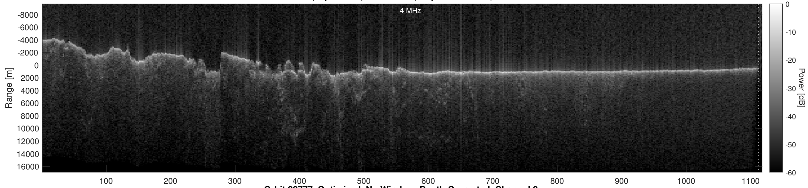
Orbit 22777, Optimized, No Window, Depth-Corrected, Channel 2
