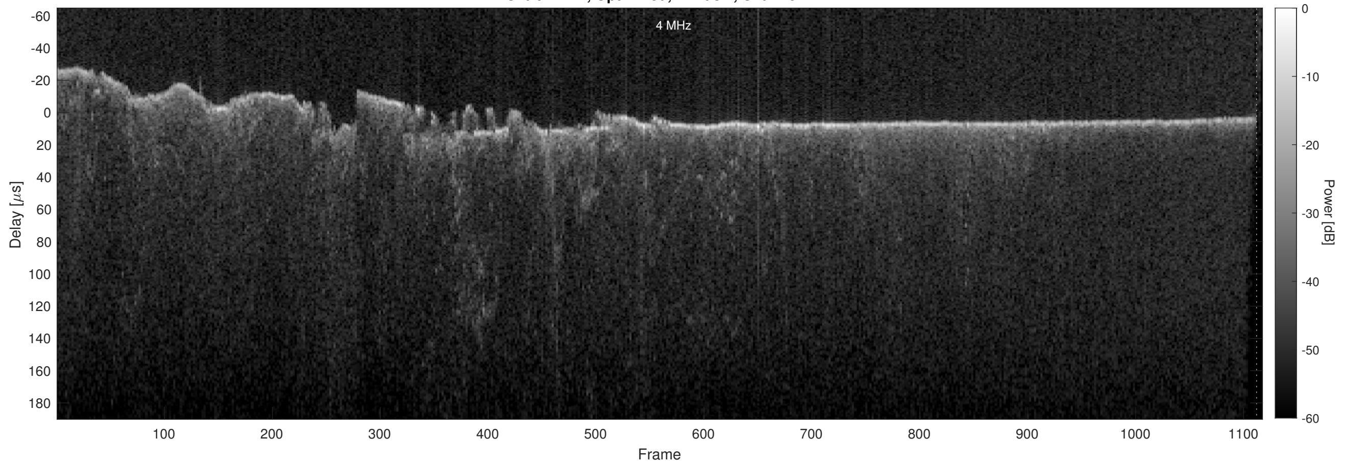
Orbit 22777, Optimized, Window, Channel 2
