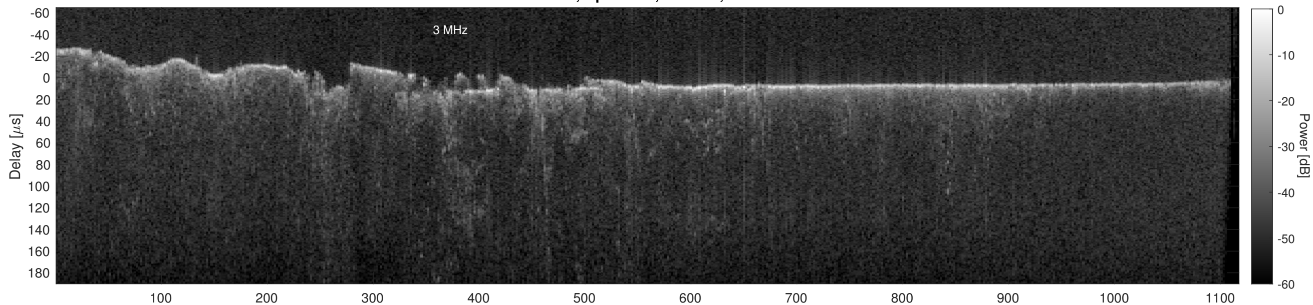
Orbit 22777, Cluttergram
