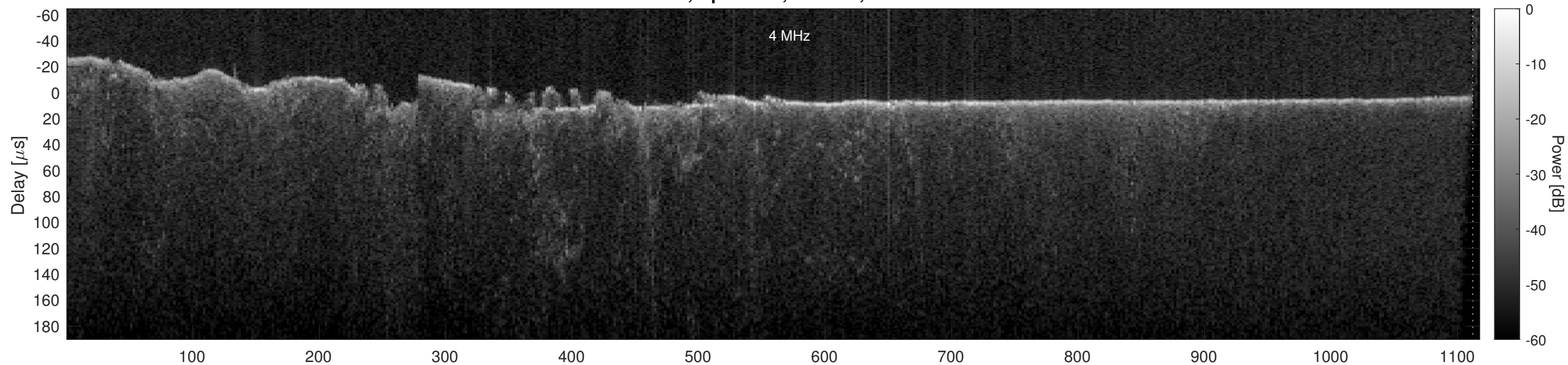
Orbit 22777, Optimized, Window, Channel 2
