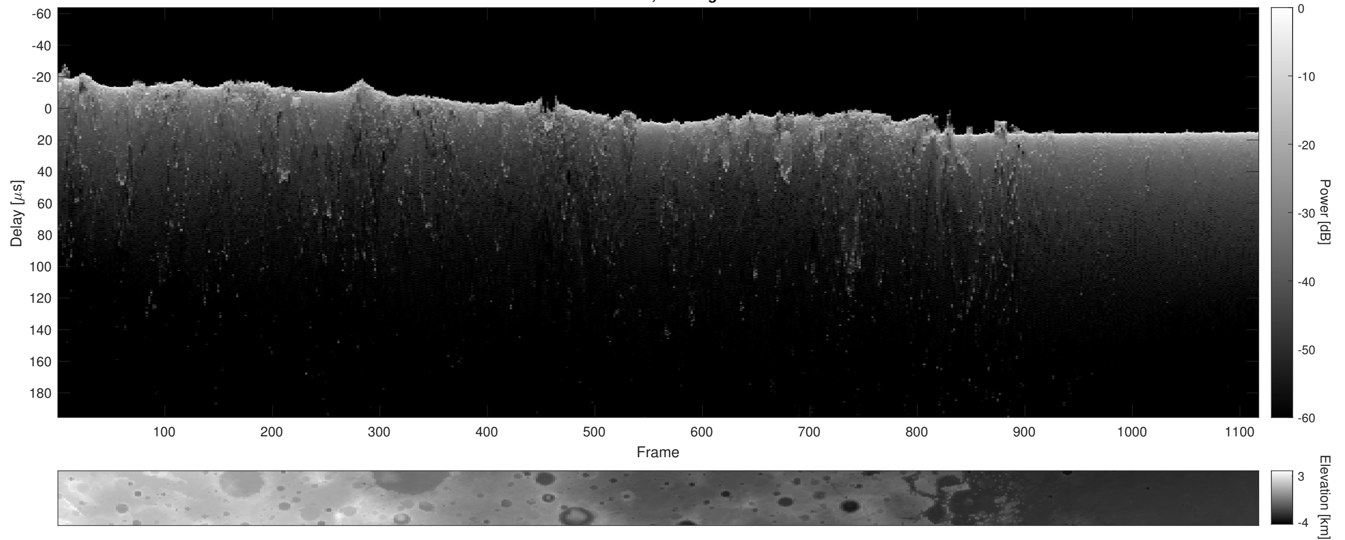
Orbit 22780, Cluttergram
