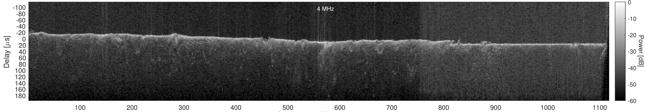
Orbit 22780, Cluttergram
