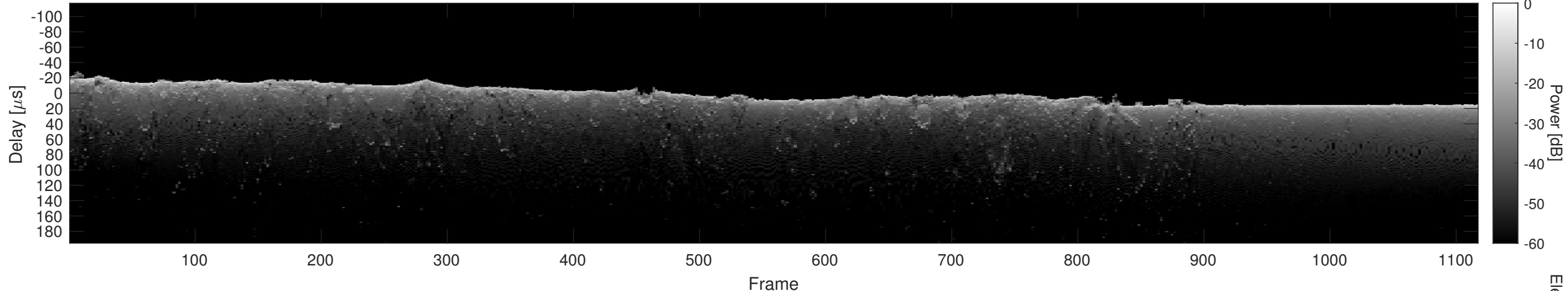
Orbit 22780, Cluttergram
