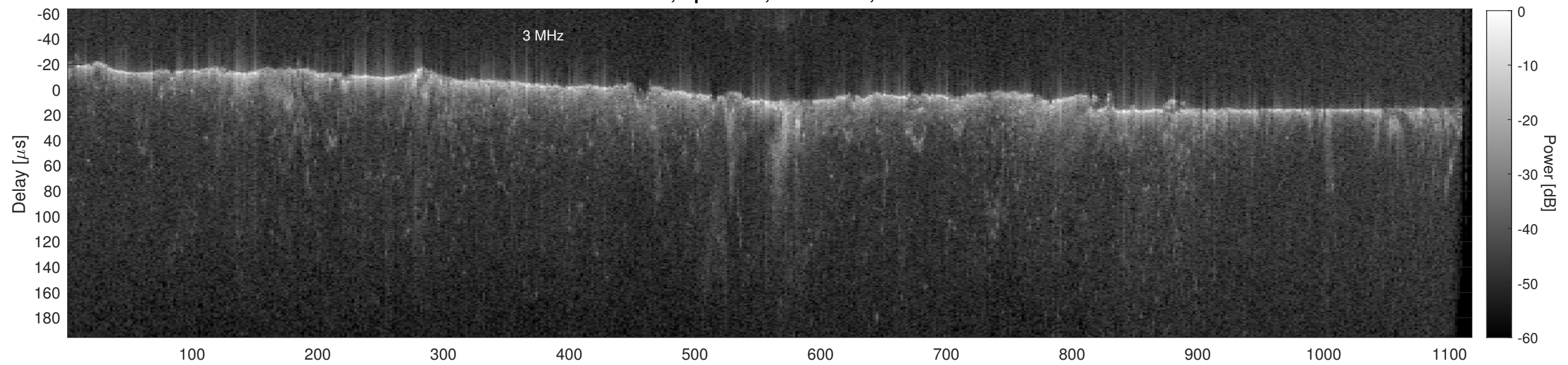
Orbit 22780, Cluttergram
