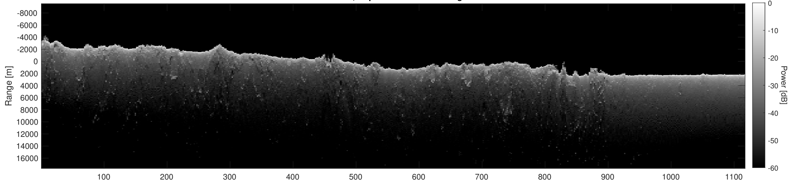
Orbit 22780, Depth-Corrected Cluttergram
