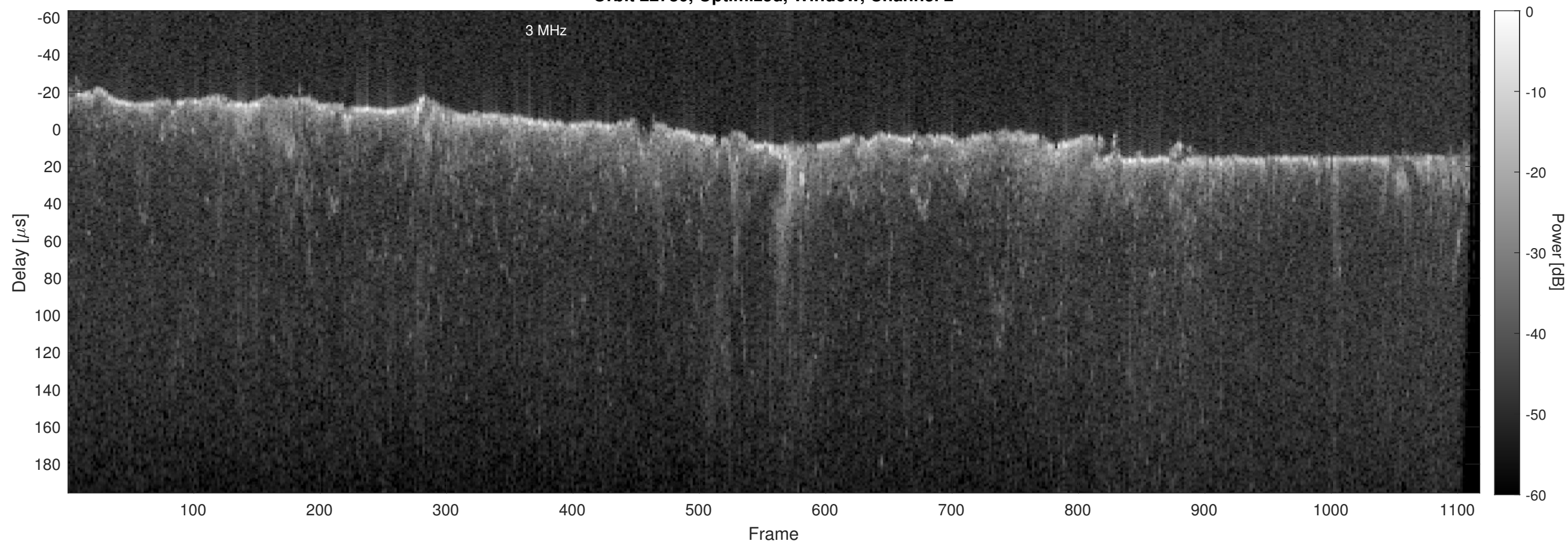
Orbit 22780, Optimized, Window, Channel 2
