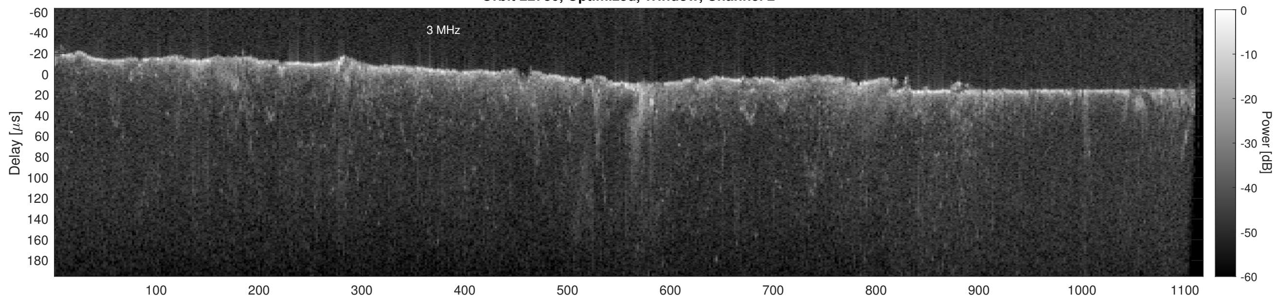
Orbit 22780, Cluttergram
