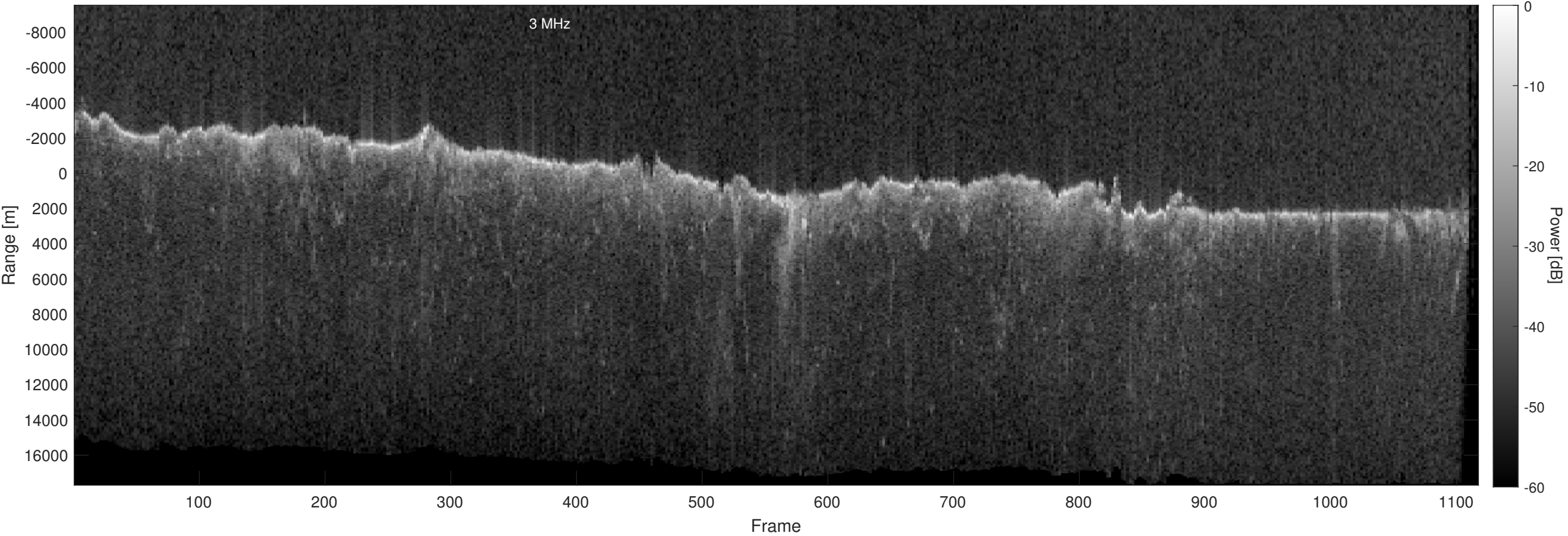
Orbit 22780, Optimized, Window, Depth-Corrected, Channel 2
