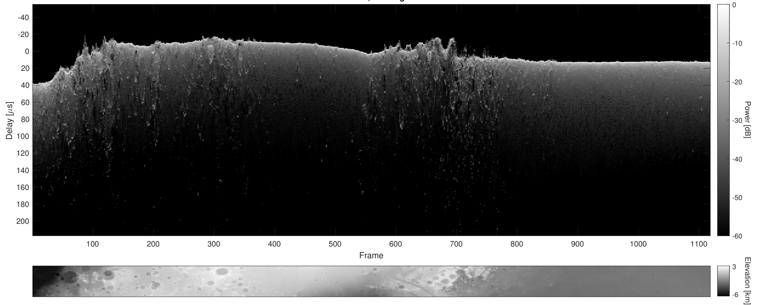
Orbit 22783, Cluttergram
