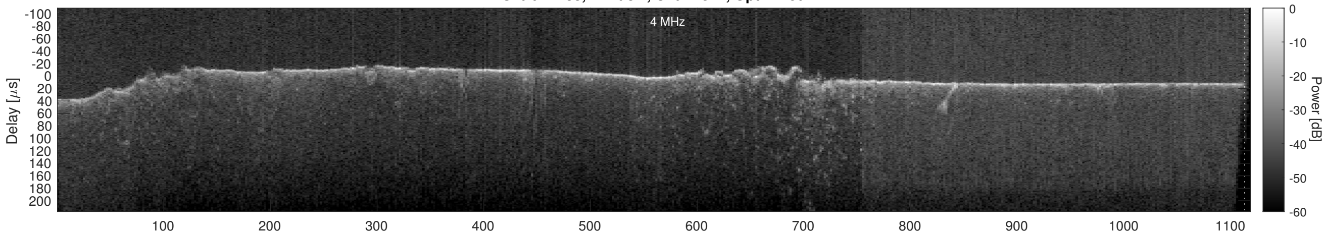
Orbit 22783, Cluttergram
