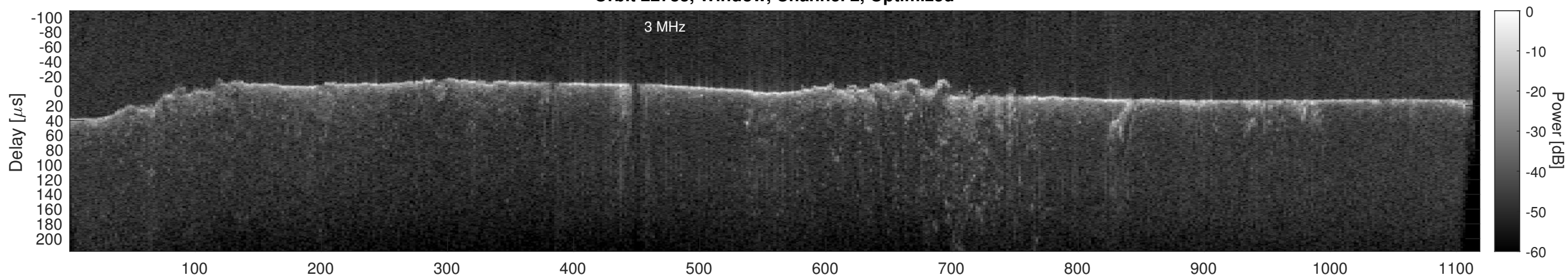
Orbit 22783, Cluttergram
