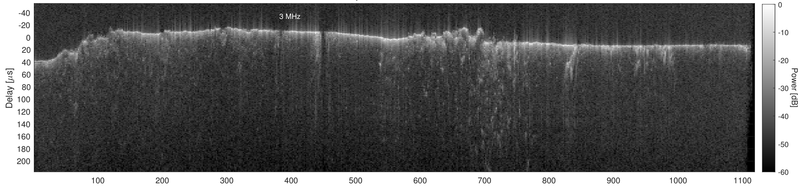
Orbit 22783, Cluttergram
