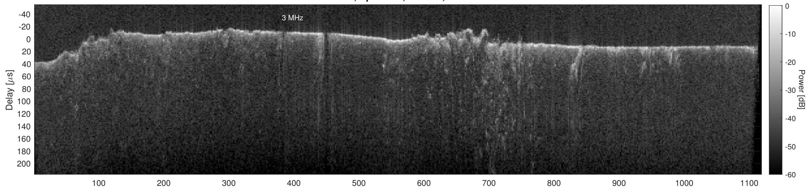
Orbit 22783, Cluttergram
