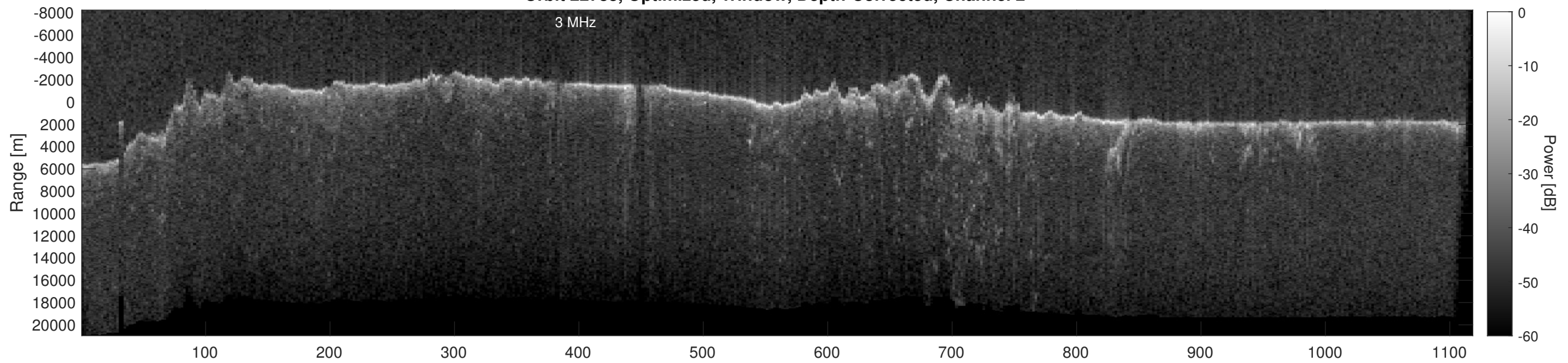
Orbit 22783, Depth-Corrected Cluttergram
