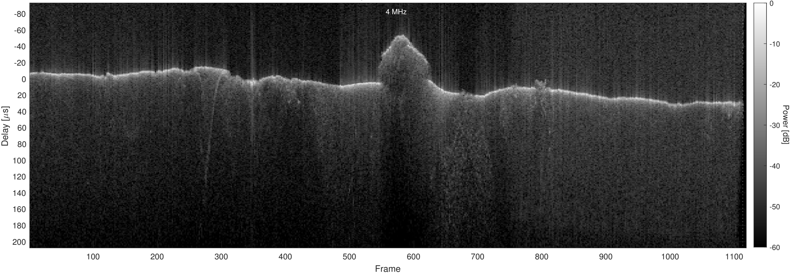
Orbit 22785, Chapman, No Window, Channel 2
