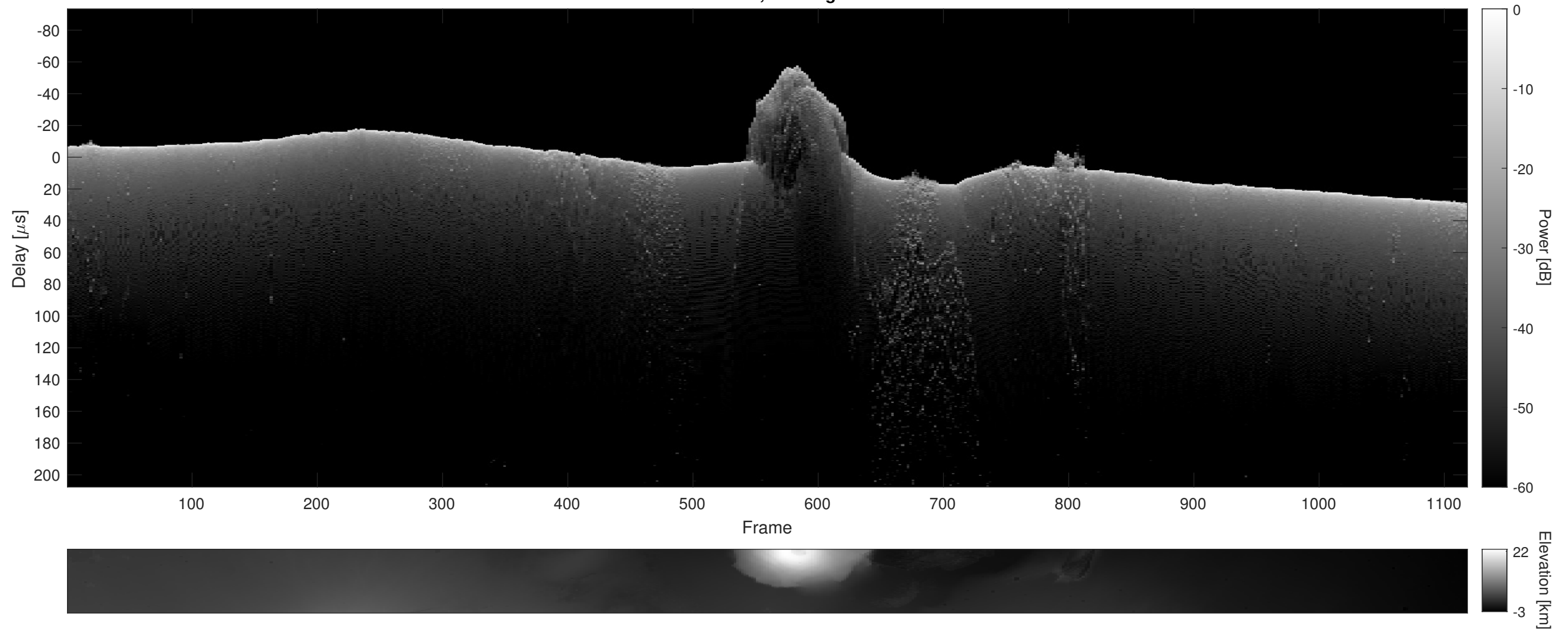
Orbit 22785, Cluttergram
