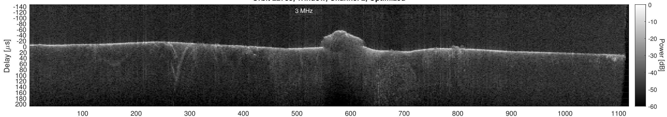
Orbit 22785, Cluttergram
