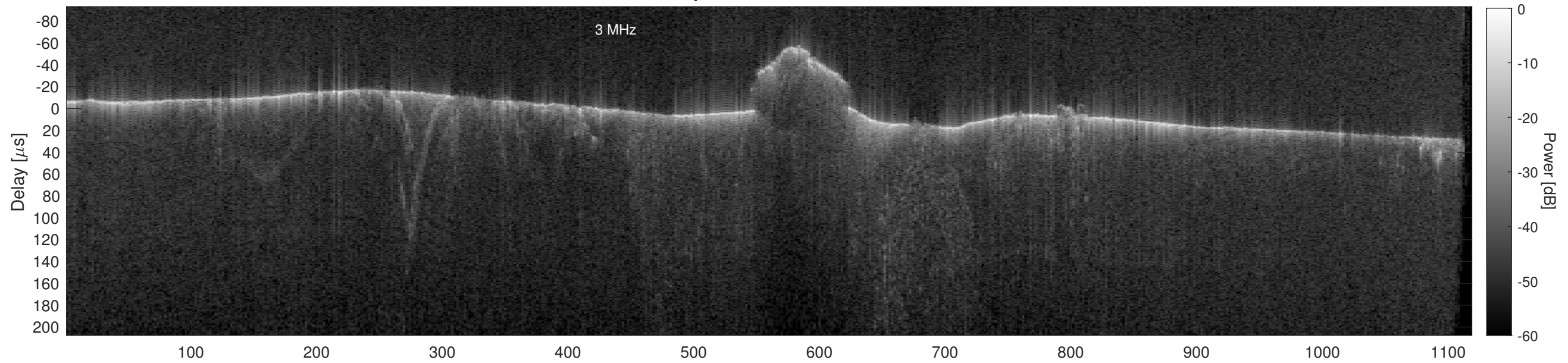
Orbit 22785, Cluttergram
