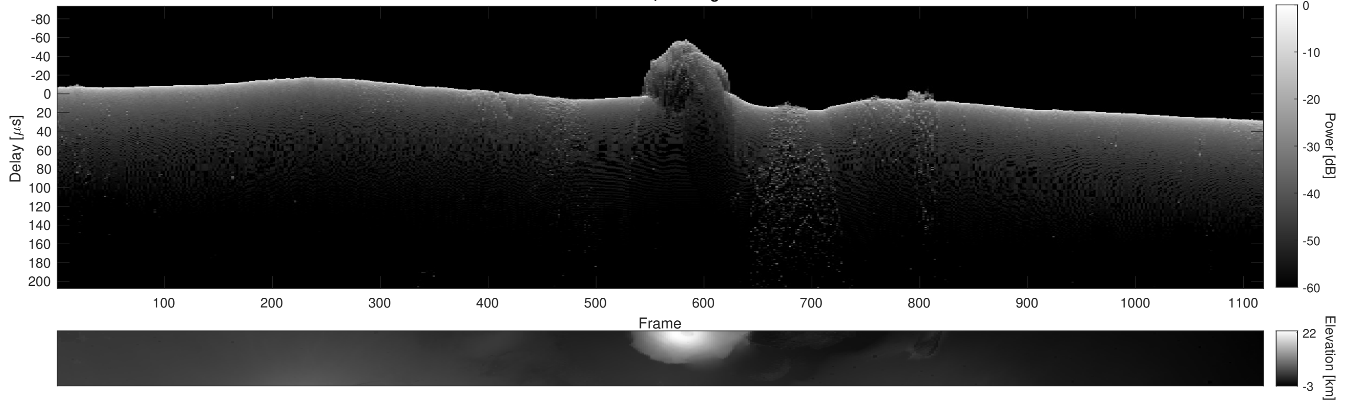
Orbit 22785, Cluttergram
