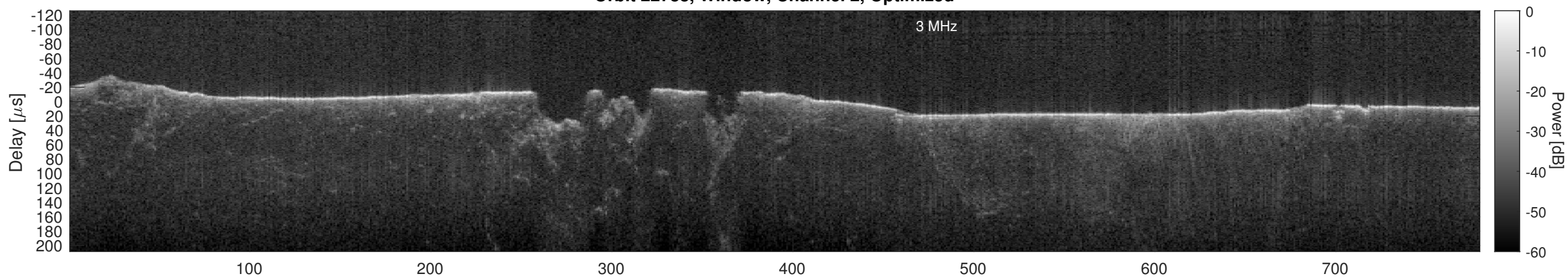
Orbit 22788, Cluttergram
